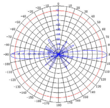
Vertical Beamwidth
